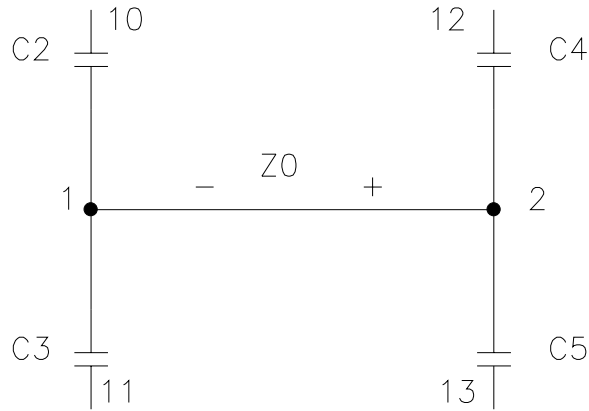
Fig. 2. Modifiable wire Z0.
