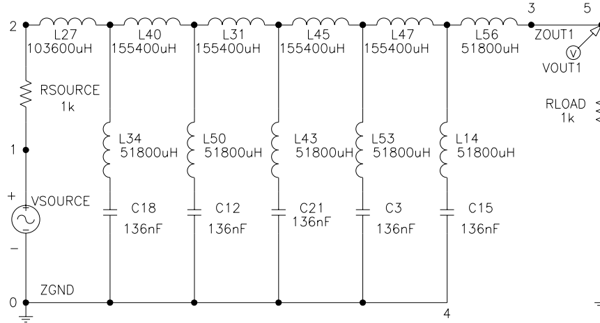
Fig. 13. Evolved Cauer (elliptic) filter topology from generation 31.
