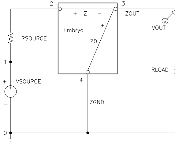
Fig. 1. One-input, one-output embryonic (initial) circuit .
