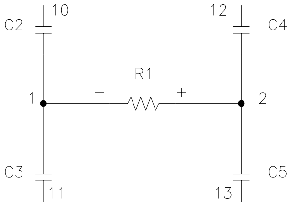
Fig. 3. Result of applying the R function.
