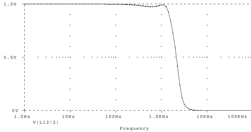
Fig. 8. Frequency domain behavior of the best circuit of generation 15.
