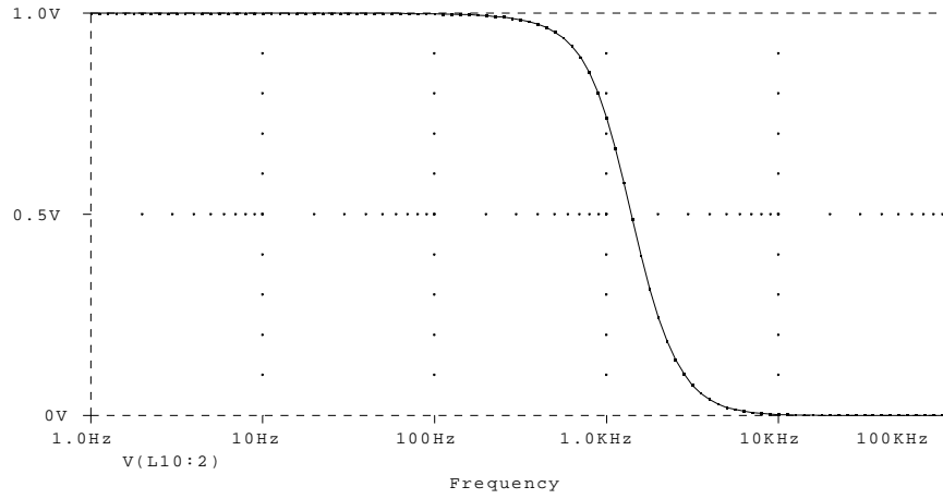
Fig. 7. Frequency domain behavior of the best circuit of generation 10.
