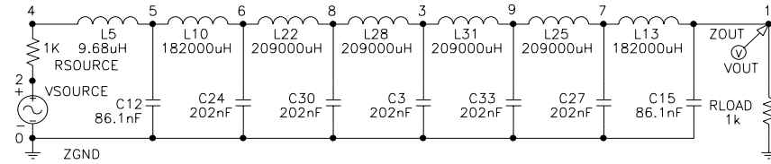
Fig. 10. Evolved seven-rung ladder lowpass filter.
