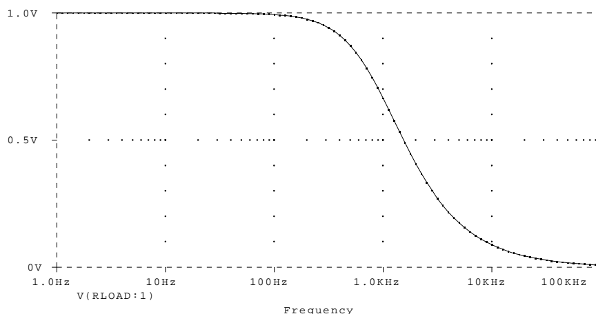
Fig. 6. Frequency domain behavior of the best circuit of generation 0.
