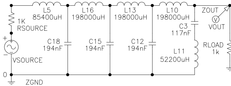
Fig. 11. Slightly modified version of the evolved lowpass filter circuit consisting of three symmetric T-sections and an M -derived half section.
