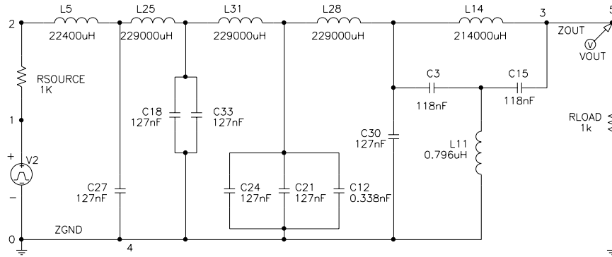
Fig. 12. “Bridged T” circuit from generation 64.
