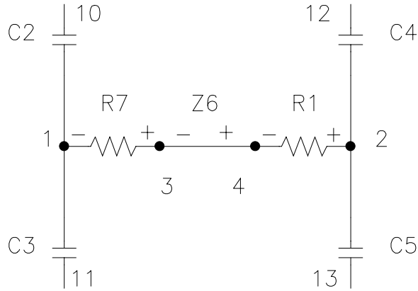
Fig. 4. Result after applying the SERIES division function.
