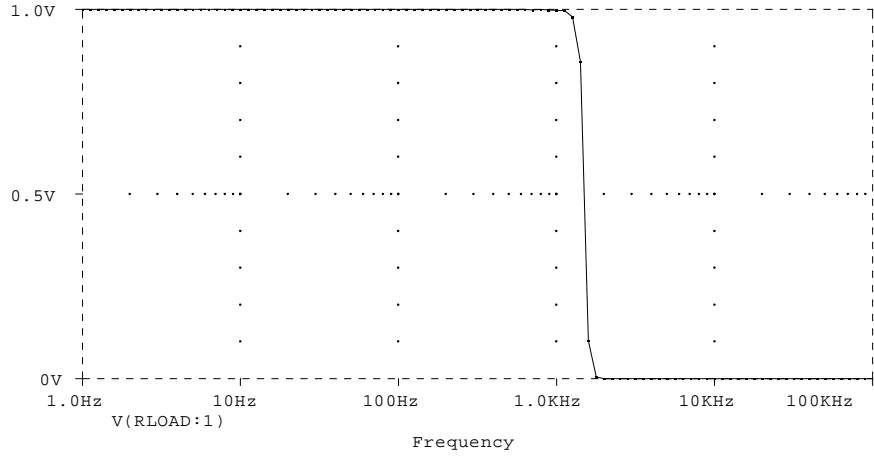
Fig. 9. Frequency domain behavior of 100%-compliant seven-rung ladder circuit from generation 49.
