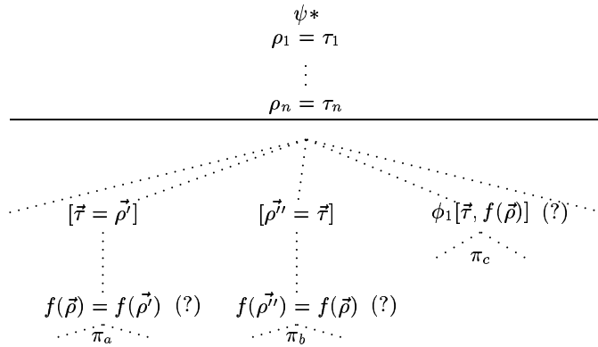
Fig. 6.1. Tableau-like figure after the deep replacement f(\vec{\tau}) := f(\vec{\rho})
