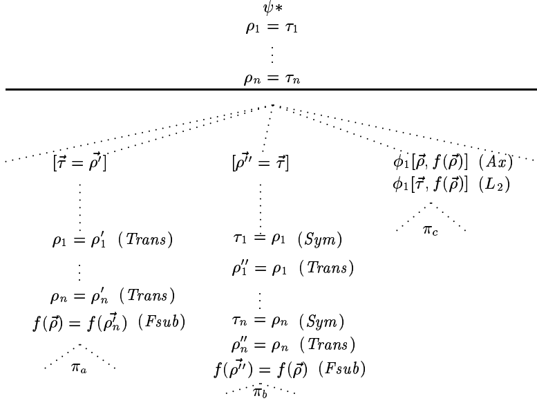
Fig. 6.2. Corrected tableau \pi_{n+1}
