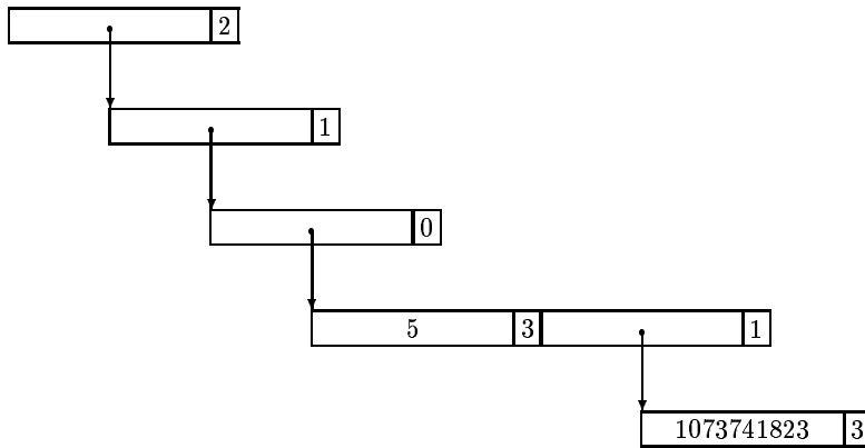
Fig. 17.1. Memory representation of the extended mixed numeral (5, 10737418231)\mathbf{01}
